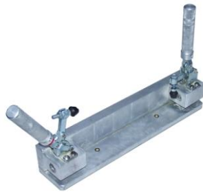
Field Drill Jig
